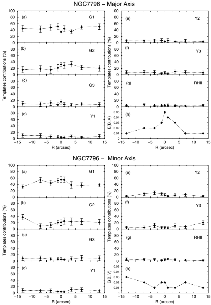
Fig. 25. Synthesis results of NGC 7796 in flux fractions as a function of the distance to the center along both photometric axes – panels a , b , c , d , e , f and g for each base component; panel h – spatial distribution of the internal reddening (like Fig. 24).
