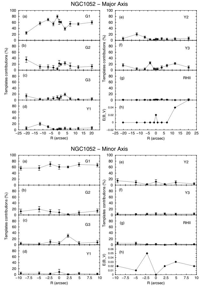
Fig. 24. Synthesis results of NGC 1052 in flux fractions as a function of the distance to the center along both photometric axes – panels a) , b) , c) , d) , e) , f) and g) for the G1, G2, G3, Y1, Y2, Y3 and RHII components respectively; panel h) – spatial distribution of the internal reddening. Note that the abscissa axis has a different scale for each plot.
